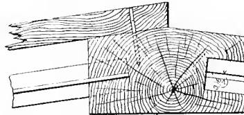
Fig. 2374. Cross Section of Ridge-pole.
